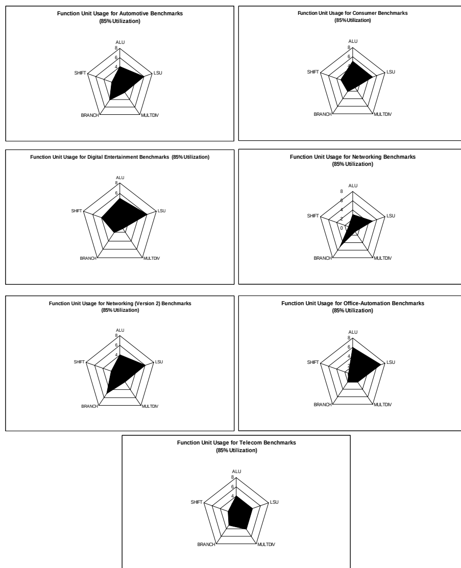
Figure 1 – Using Kiviatt Graphs to Represent Functional Unit Distribution (85 % Utilization)
